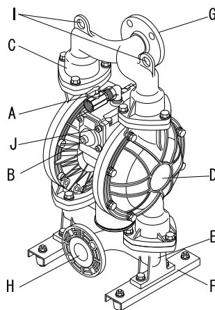
NDP-40BS□ NDP-40BF□
