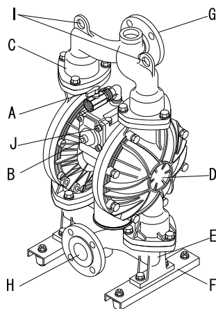
NDP-40BA□
