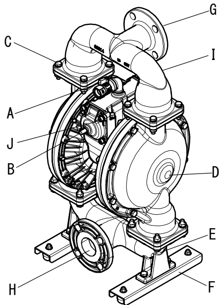
NDP-500BS□
